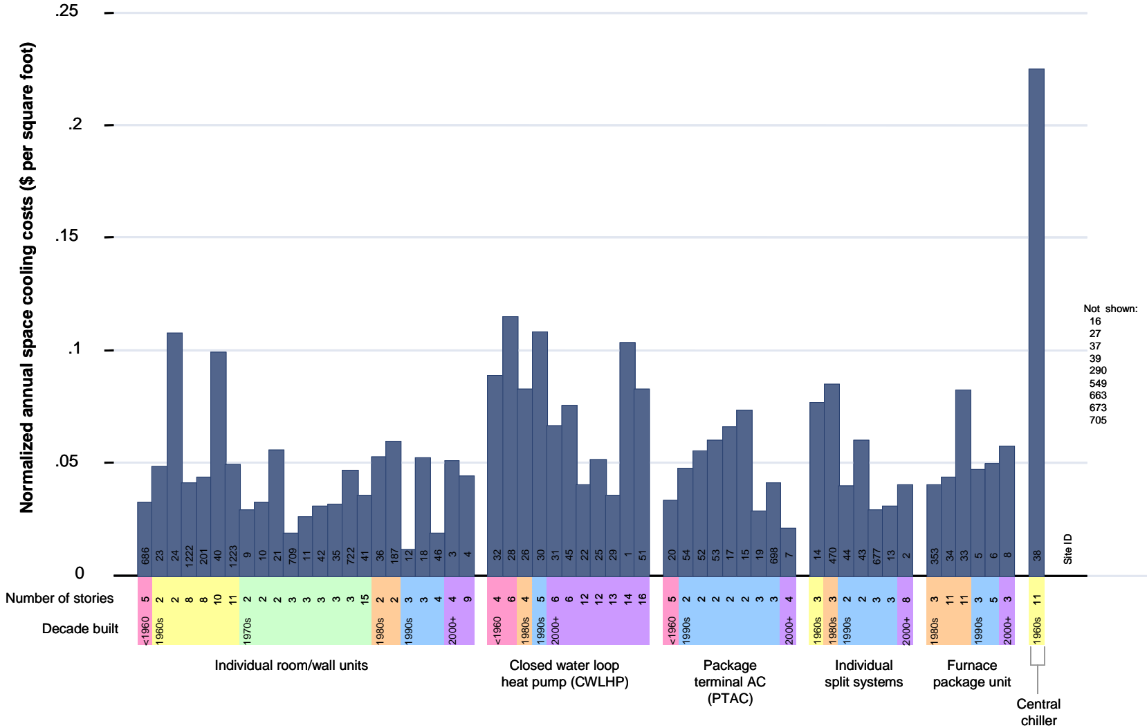
FIGURE 5, WEATHER NORMALIZED ESTIMATED ANNUAL SPACE COOLING COSTS BY SITE, SORTED BY COOLING SYSTEM TYPE, DECADE OF CONSTRUCTION AND NUMBER OF STORIES.
