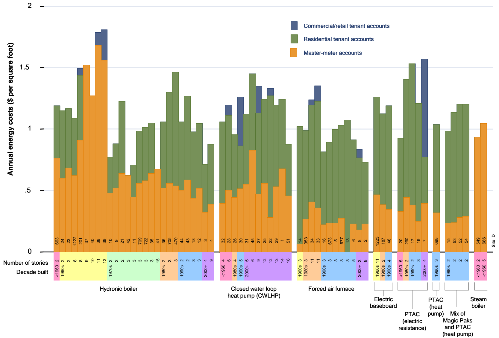
FIGURE 2, ANNUAL ENERGY COSTS BY SITE, SORTED BY HEATING SYSTEM TYPE, DECADE OF CONSTRUCTION AND NUMBER OF STORIES.
